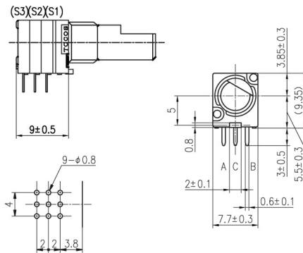
TP70TF5161(S) (S)=Sealed with O-ring between shaft and bushing
